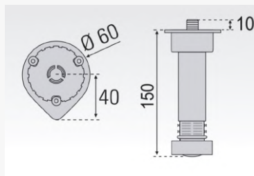
Dimensions techniques
